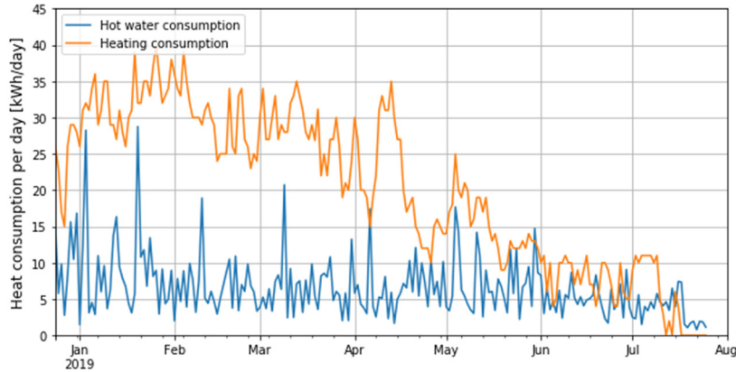
Figure 3-5 The daily energy use for space heating and domestic hot water.
