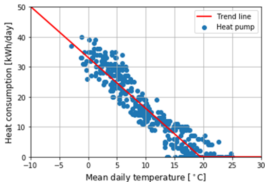
Figure 3-2 Daily heating consumption as a function of the mean daily outdoor temperature.
