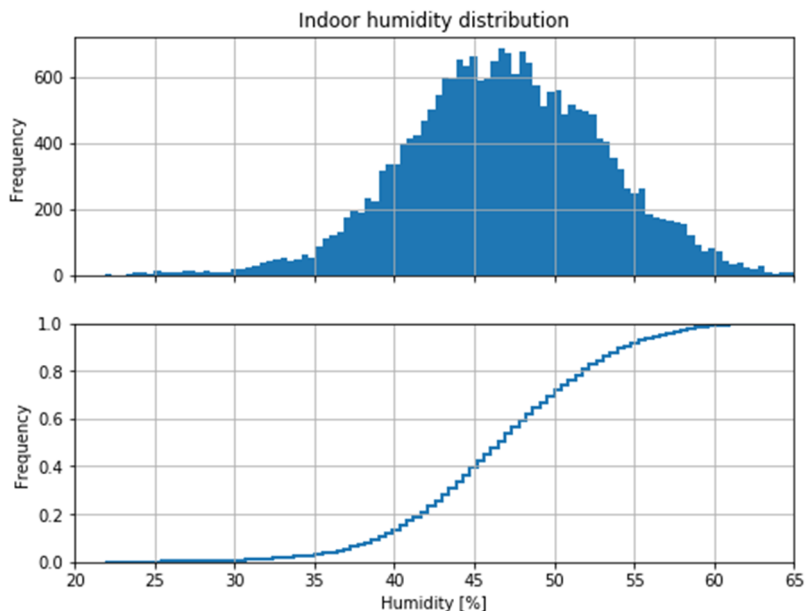
Figure 4-2 The indoor humidity in the house during the measuring period.
